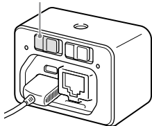
MASTER/CLIENT switch
