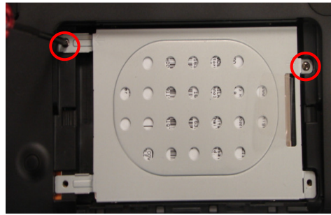
Step 5. Using the enclosed magnetic screwdriver, remove the two (2) screws securing the Hard Drive Assembly. Put aside the Hard Drive Screws to re-secure the Hard Drive later in the procedure.
