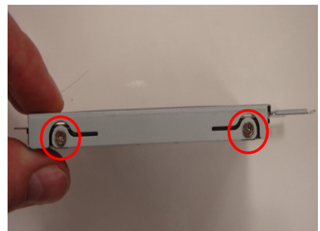
Step 9. Holding the edge of the Hard Drive, remove each screw. Put aside the Bracket Screws to secure the Bracket to the Hard Drive later in the procedure.
