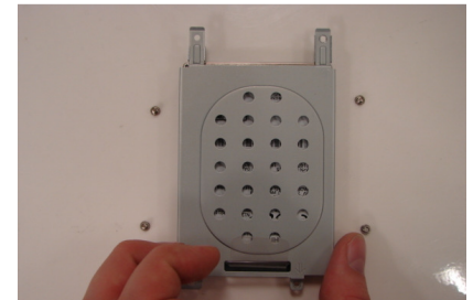
Step 12. Place the Hard Drive bracket over the new Hard Drive.
