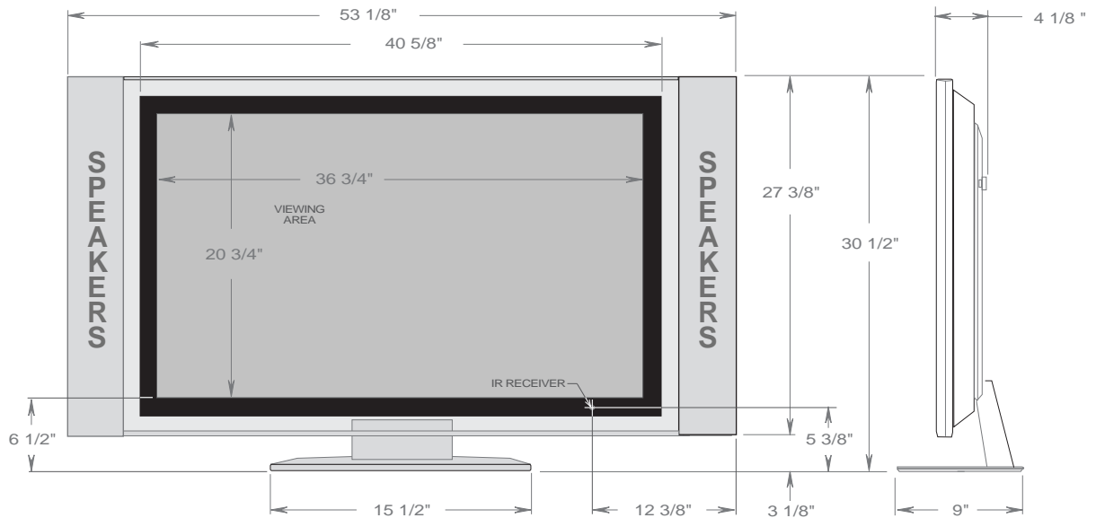
FRONT VIEW
